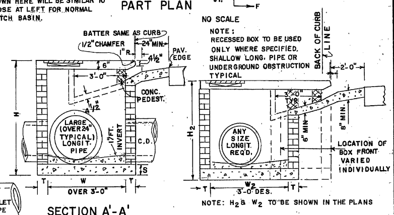
SECTION A-A (WITH LARGE LONGITUDINAL PIPE)
