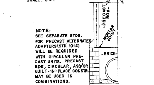
PRECAST BOX ON BRICK (HALF-SECTION)
