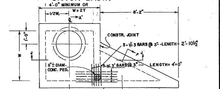
PART PLAN
