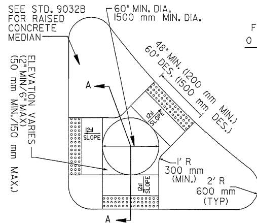
CONCRETE ISLAND WITH ELEVATED CUT THROUGH
