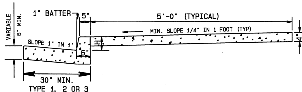
TYPICAL SECTION 30" CURB & GUTTER WITH 4" SIDEWALK
