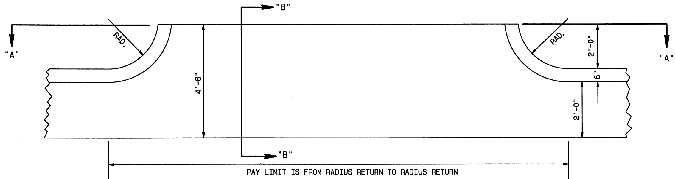
PLAN
