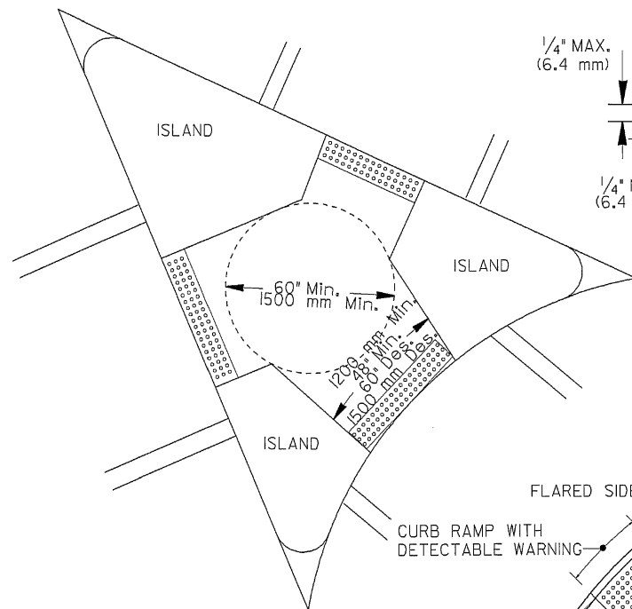
CONCRETE ISLAND WITH ELEVATED CUT THROUGH
